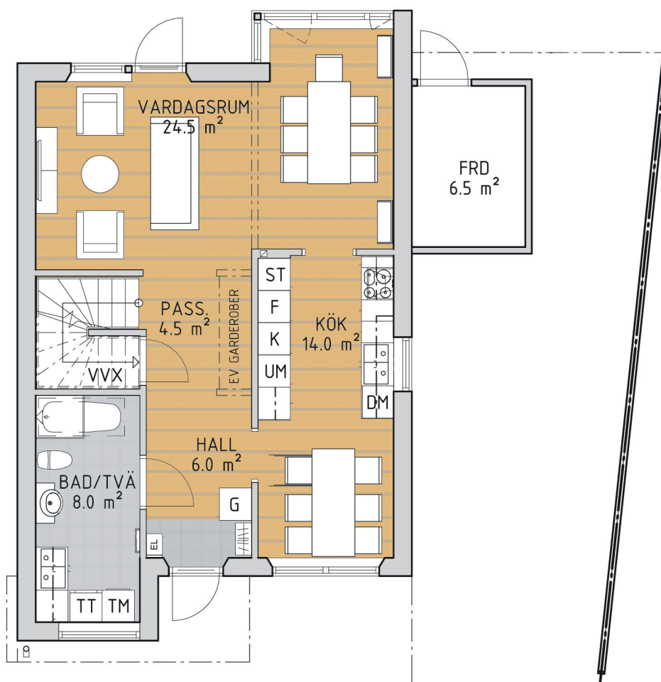
Plan 1
