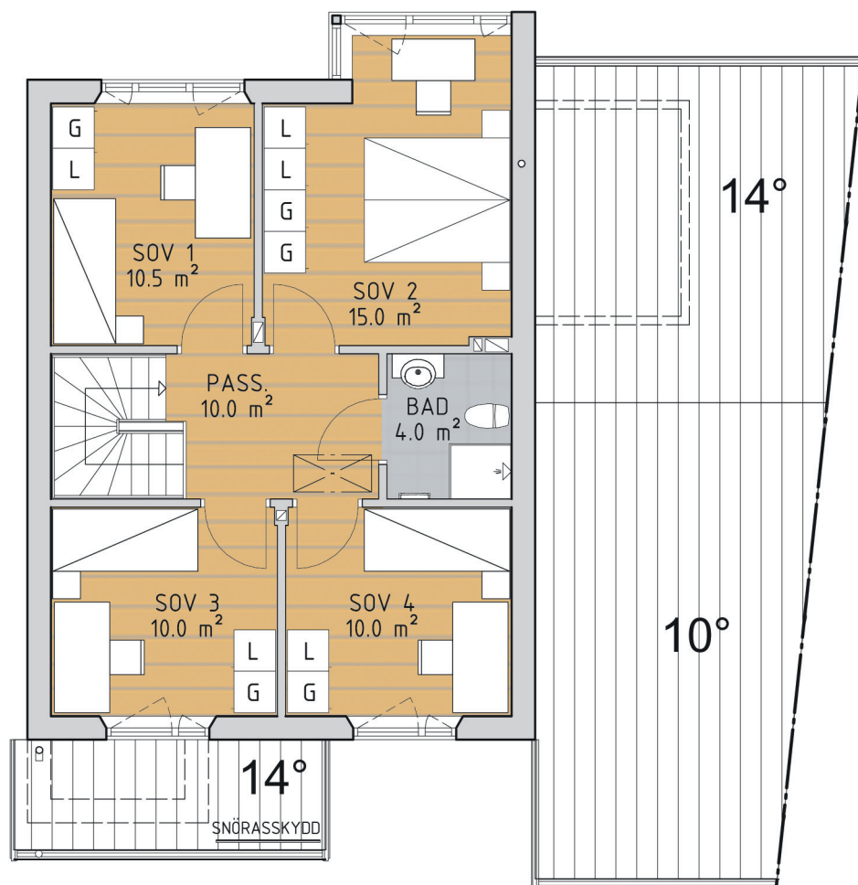
Plan 2
