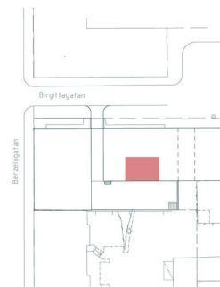
Situationsplan
